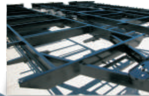
Additional Welds Create Camber in the Chassis for Greater Load Carrying Capacity
