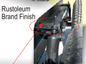
Shock Mounts-All Wheels (Except 17C)
