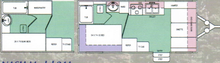
NASH Model 24A
