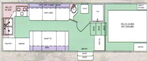
NASH Model 24-5K
