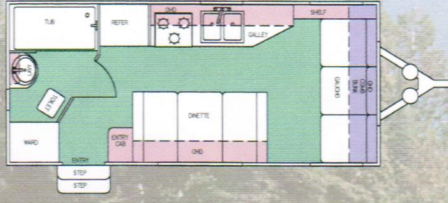
NASH Model 22G
