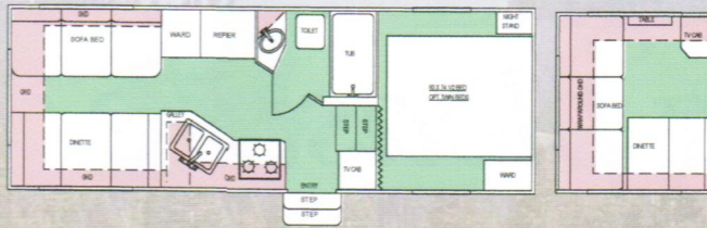
NASH Model 25-5M
