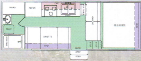
NASH Model 24-5K
