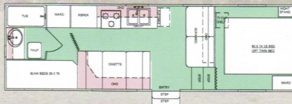
NASH Model 25-5M
