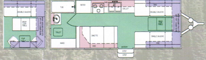
NASH Model 22GQ
